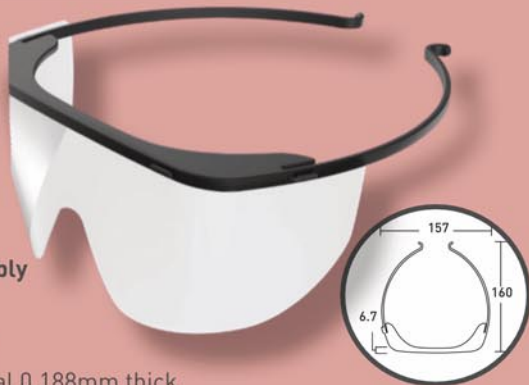
EYEWEAR GEOMETRY Units:mm
