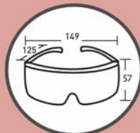
EYEWEAR GEOMETRY Units:mm
